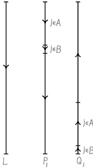
Fig. 2. The orders L , P_j and Q_j .
