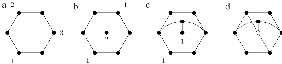
Fig. 4. Coloring of three vertices with colors 1, 2 and 3 in (a), (b) and (c) or an extra vertex of degree 5 in (d) forces a coloring of the 6-cycle with a sequence (1, 2, 3, 1, 2, 3) in cyclic order.
