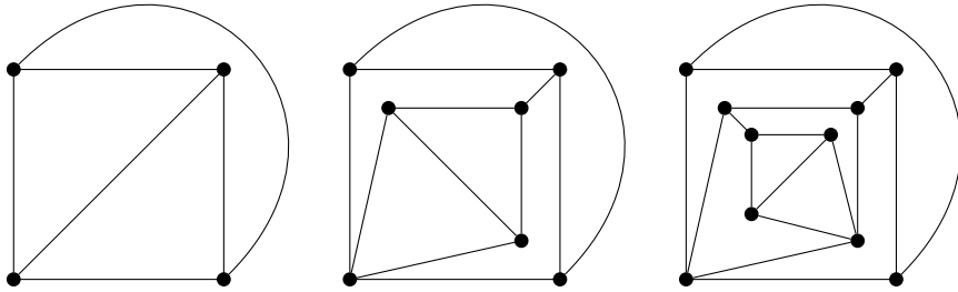
Fig. 3. First three 4-critical graphs from the family described by Thomas and Walls [24].
