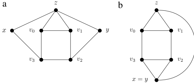
Fig. 1. Triangle adjacent to a 4-face in Lemma 10.
