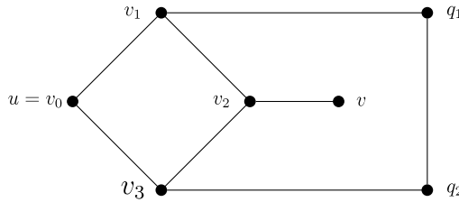
Fig. 2. Configuration from Theorem 6.
